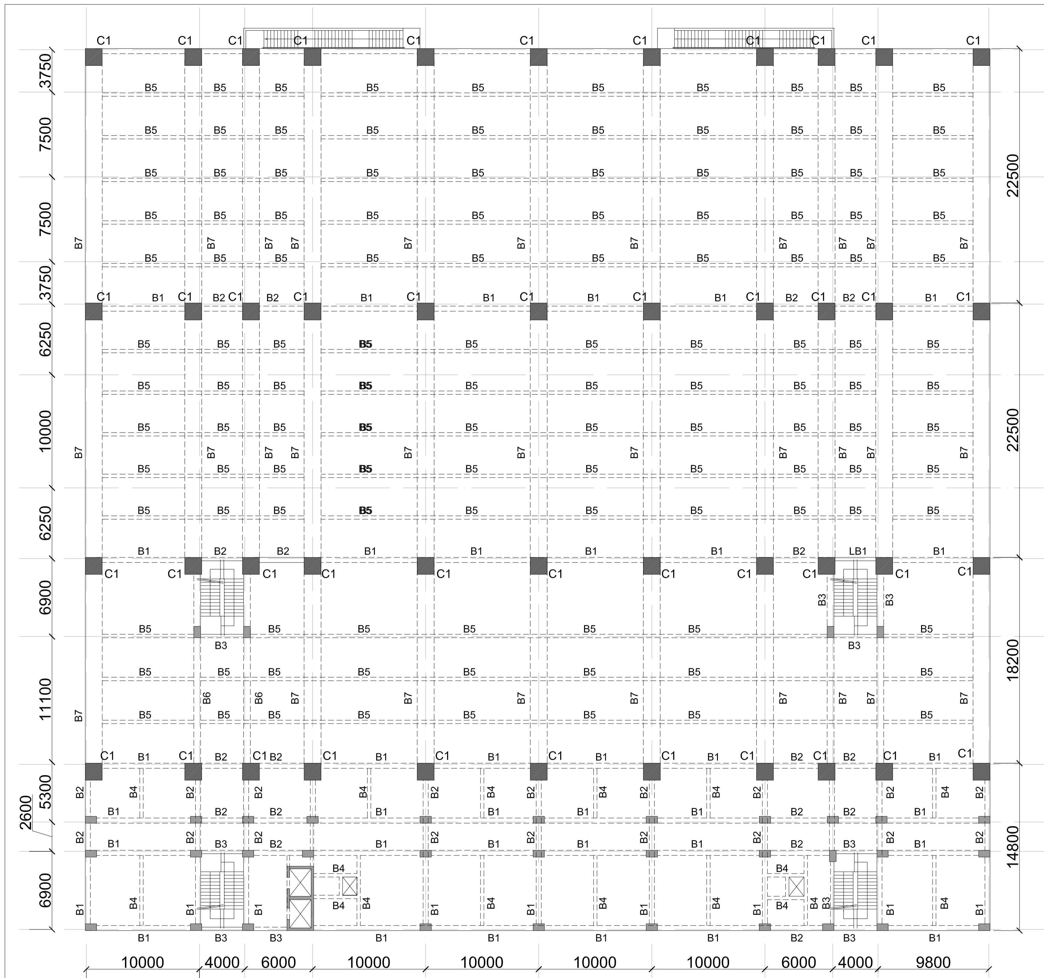
FIRST FLOOR LVL. FRAMING PLAN NOTE:- ALL COLUMN SIZE ARE (600X1000) UNLESS NOTED OTHERWISE C1 = 1500X1500
