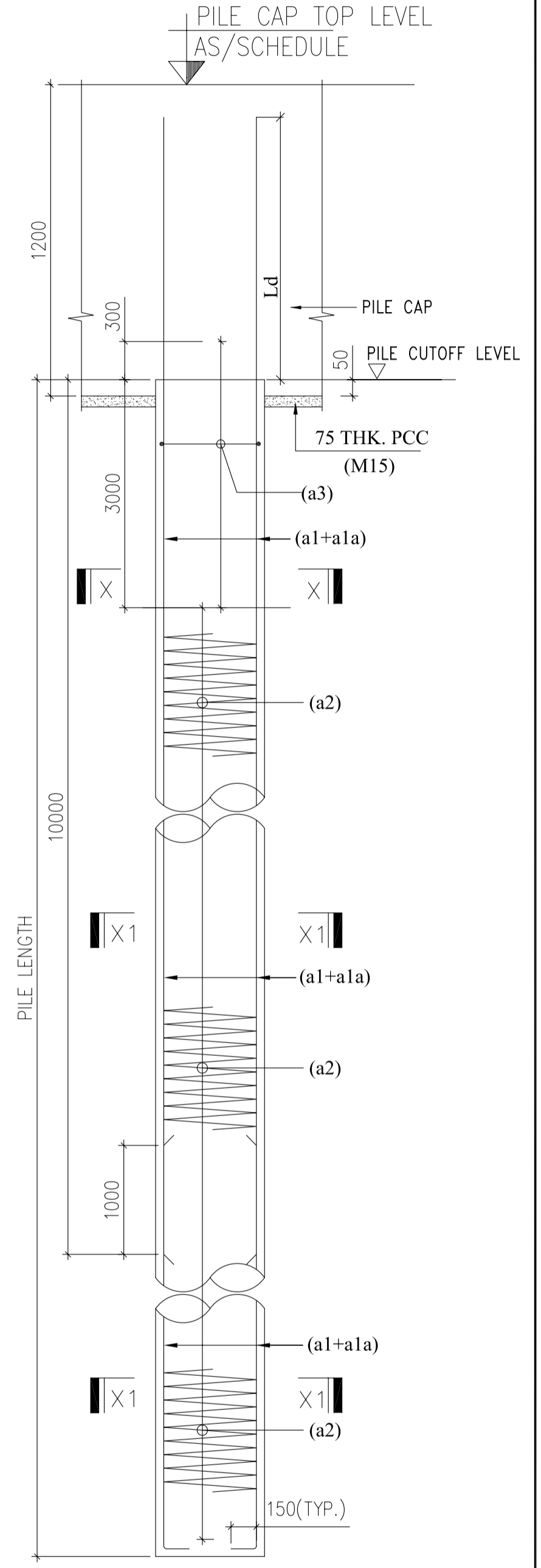
DETAIL OF PILE - PC1 SCALE 1:50
