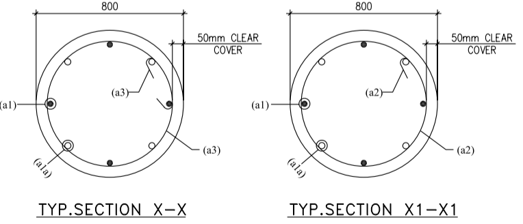
DETAIL OF PILE - PC1 SCALE 1:50
