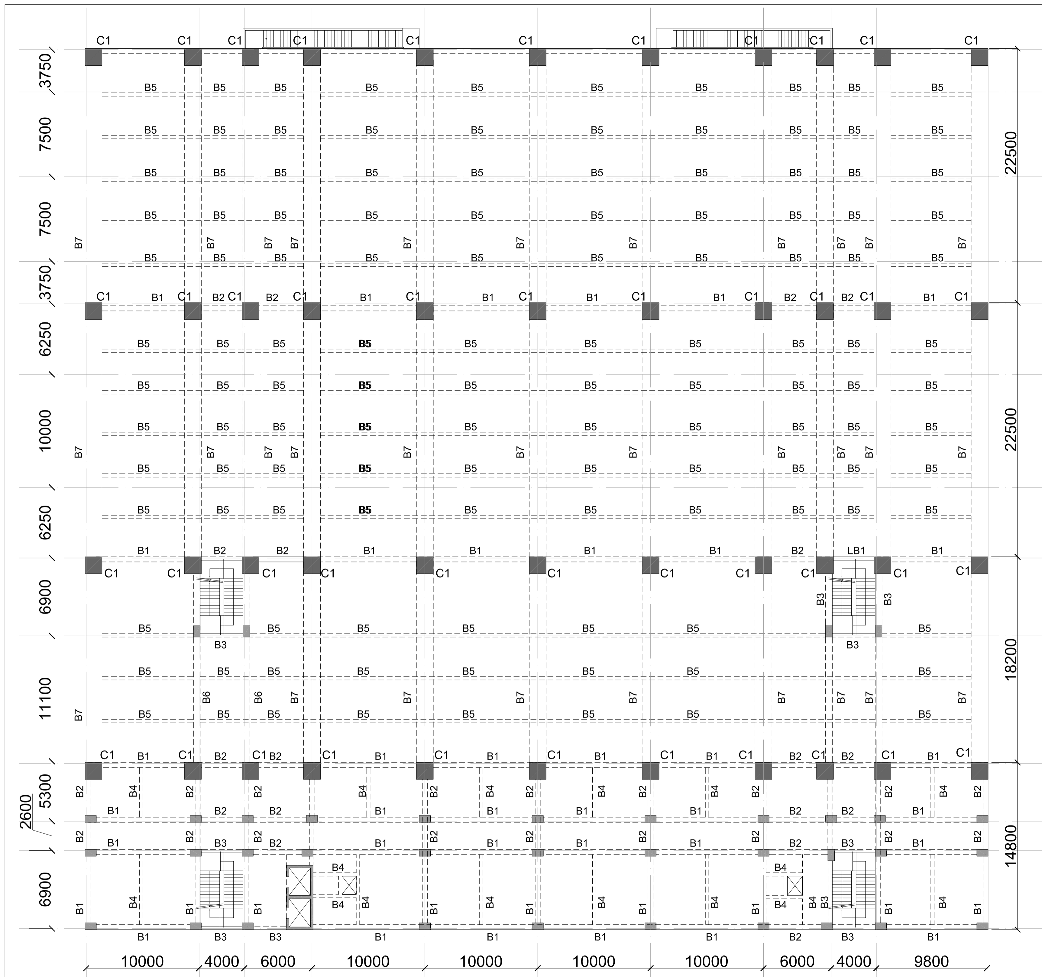
TERRACE LVL. FRAMING PLAN NOTE:- ALL COLUMN SIZE ARE (600X1000) UNLESS NOTED OTHERWISE C1 = 1500X1500
